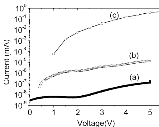
FIG. 2. Leakage current characteristics of the MIS structures: (a) with a HfO 2 /SiO 2 stack tunnel layer annealed at 600 °C for 30 min; (b) with a HfO 2 /SiO 2 stack tunnel layer annealed at 800 °C for 45 min; (c) with a HfO 2 tunnel layer only and annealed at 800 °C for 45 min.
