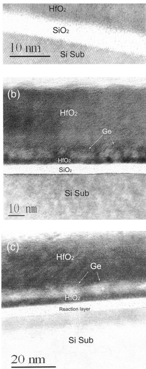
FIG. 1. Cross-sectional HRTEM images of the MIS structure with Ge nanocrystals embedded in HfO 2 dielectric with a HfO 2 /SiO 2 stack tunnel layer annealed at 600 °C for 30 min (a), and annealed at 800 °C for 45 min (b); (c) with a HfO 2 tunnel layer only and annealed at 800 °C for 45 min.
