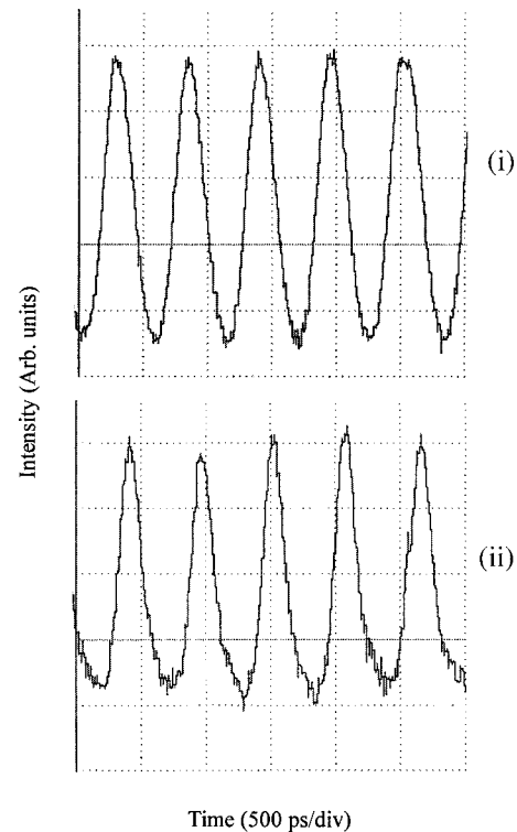
Fig. 7. Waveforms of output pulse trains at wavelengths of (i) 1548.9 and (ii) 1548.4 nm.
