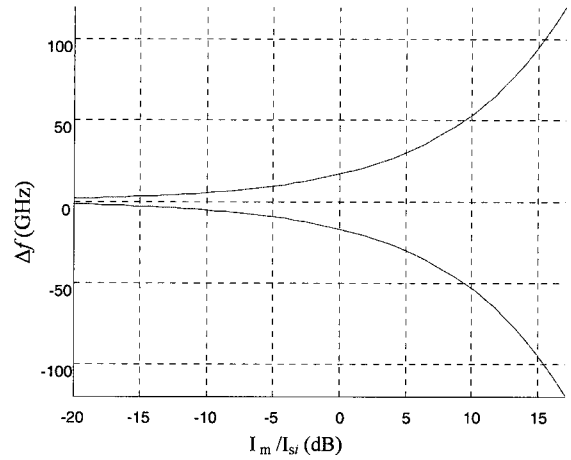
Fig. 1. Frequency locking range versus injection ratio I_m/I_{s_i} .
