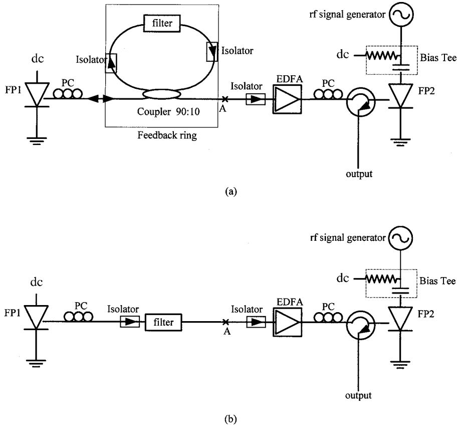
Fig. 2. (a) Experimental setup for external injection seeding with feedback to the master FP laser source. (b) Experimental setup for external injection seeding without feedback to the master FP laser source.
