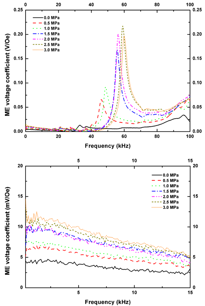
FIG. 5. (Color online) Frequency dependence of ME voltage coefficient as a function of preloading stress for a PMN-PT single crystal/Terfenol-D ME sensor. (Inset: a magnified picture of low frequency region.)
