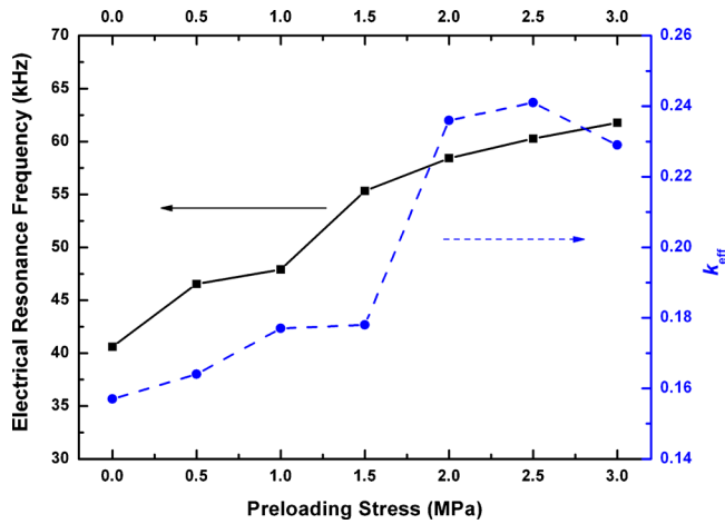
FIG. 4. (Color online) Electrical resonant frequency and k_{\text{eff}} of a PMN-PT single crystal/Terfenol-D ME sensor obtained in an impedance measurement as a function of preloading stress.
