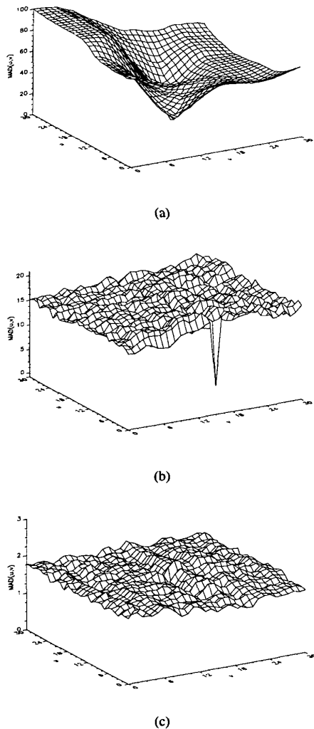
Figure 1. MAD Error Surface for three different blocks.
