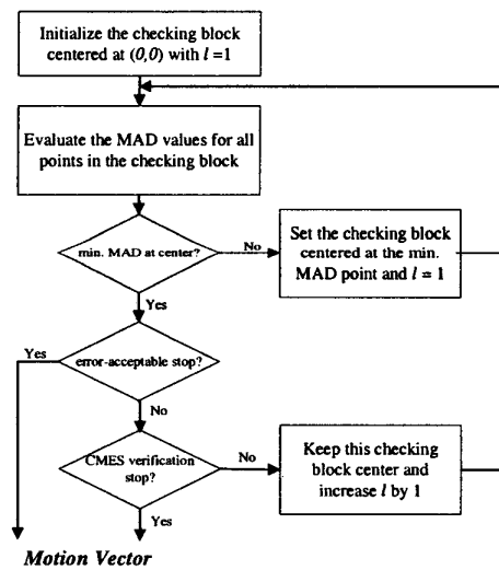
Figure 5. Block diagram of the new BBGDS algorithm
