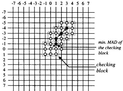
Figure 2. Example of the BBGDS search procedure, where motion vector (3, -4) is found.
