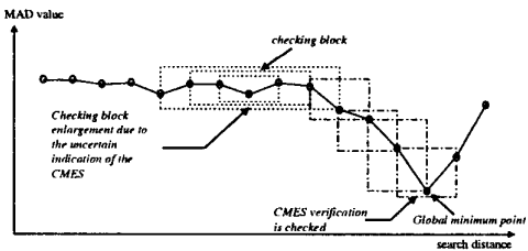
Figure 4. Reliable search through the CMES.
