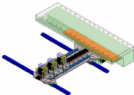
Fig. 2 End Supported Type Motor
