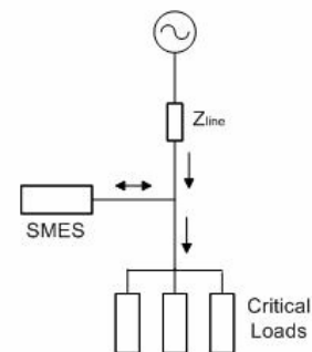
Fig. 5. SMES system for protection of distributed critical loads
