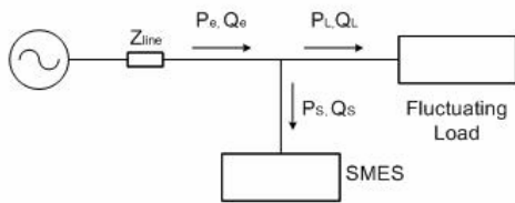
Fig. 4. Schematic diagram to compensate for fluctuating load
