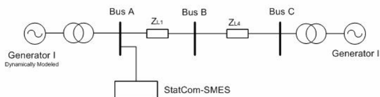
Fig. 3. Schematic improving FACTS performances using SMES
