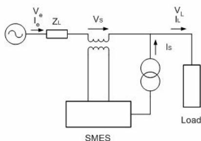
Fig. 6. Configuration of an asymmetrical compensation system with SMES
