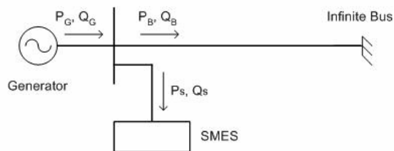
Fig. 2. Schematic diagram of an SMES unit for damping system oscillations
