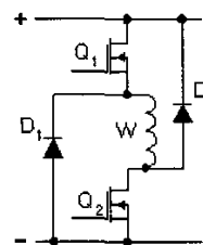
Fig. 1. Schematic diagram of a phase branch in topologies of SRM drives
