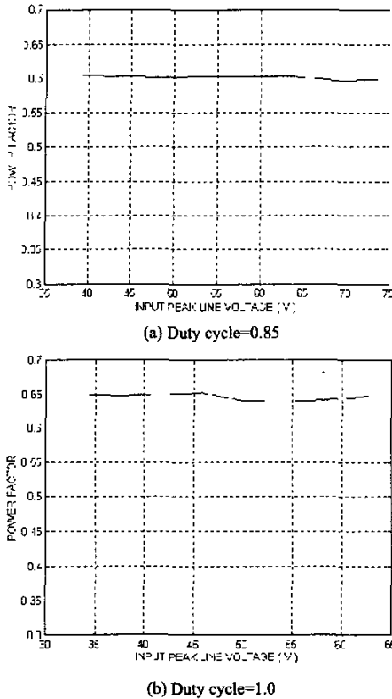
Fig. 13 Changes of power factor with input voltage at soft chopping
