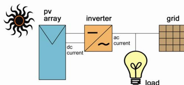
Figure 1: General schematic diagram of Grid-connect BIPV system
