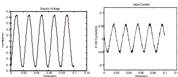
Figure 4(c) Figure 4(d) Figure 4: Discharging operation
