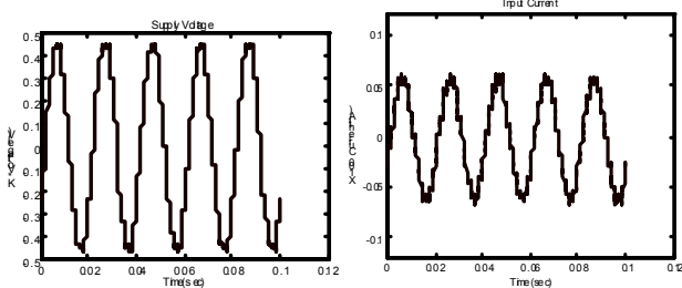
Figure 3(a) Figure 3(b) Figure 3: Charging operation
