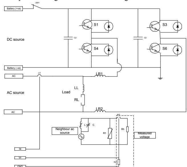
Figure 1 -- System Configuration
