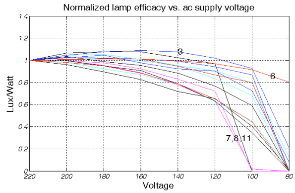
Fig. 5: Normalized lamp efficacy vs. ac supply voltage.
