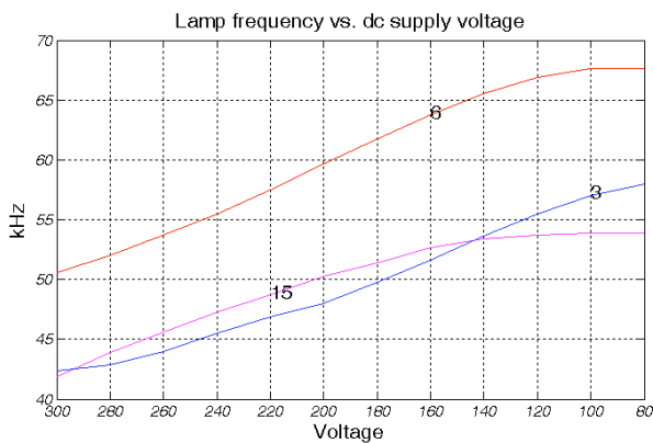
Fig. 11: Lamp frequency vs. dc supply voltage.
