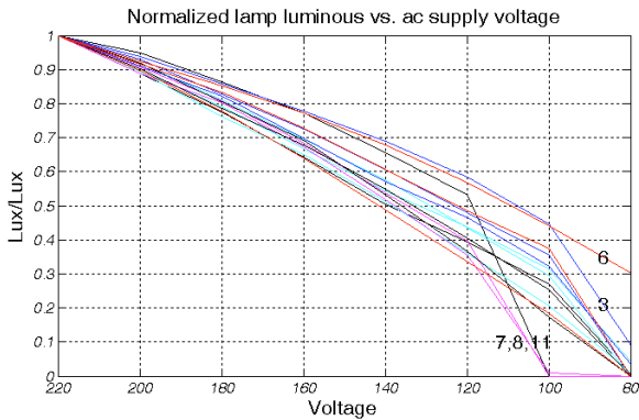
Fig. 3: Normalized lamp luminous vs. ac supply voltage.
