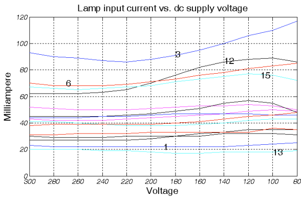
Fig. 9: Lamp input current vs. dc supply voltage.
