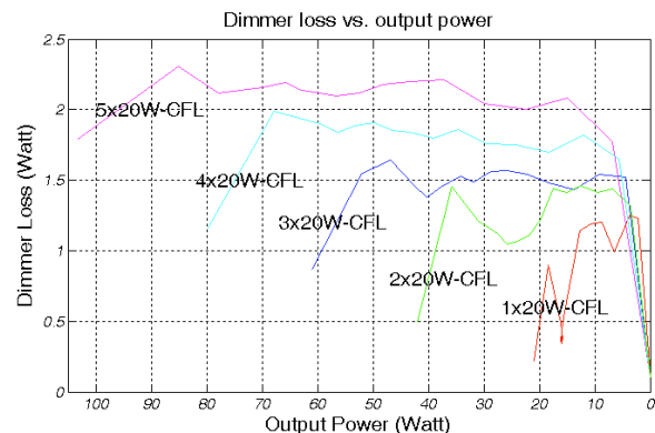
Fig. 15: Dimmer loss vs. output power for different loads
