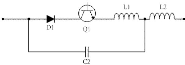
Fig. 2: Ac chopper CFL dimmer proposed by Yao in 2003
