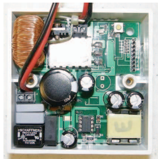
Fig. 14: Evaluation board of 100 W CFL light dimmer
