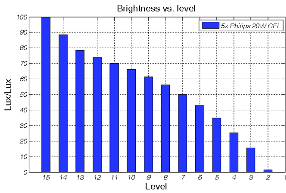
Fig. 16: Brightness vs. level
