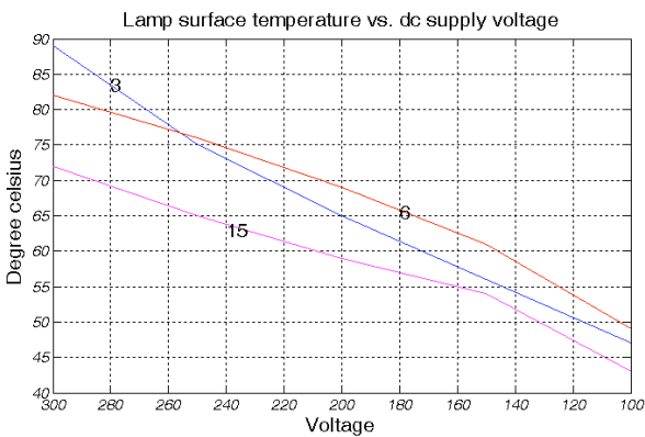
Fig. 10: Lamp surface temperature vs. dc supply voltage.
