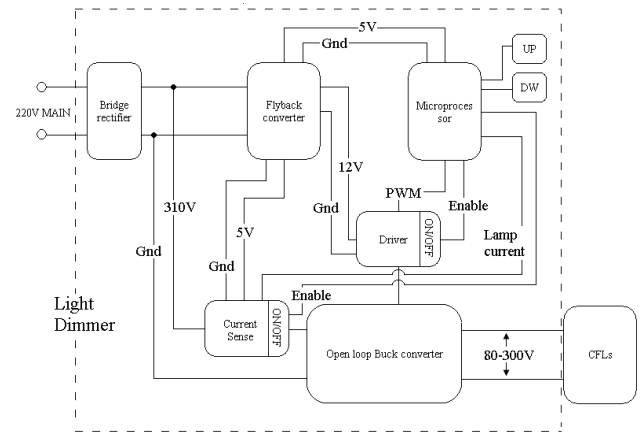
Fig. 13: Block diagram of the light dimmer
