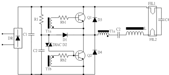
Fig. 1: Typical electronic ballast circuit with voltage fed configuration [4,5] employed in most of the CFL available in the market
