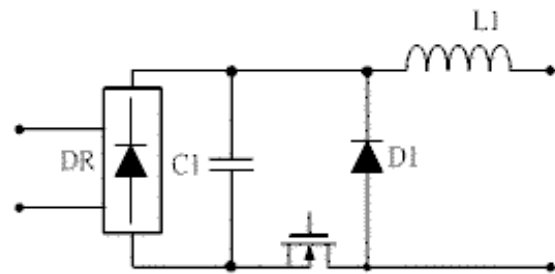
Fig. 12: Open loop buck converter as an adjustable dc source
