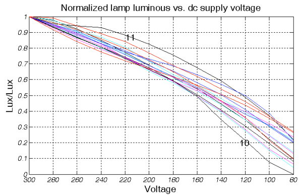
Fig. 6: Normalized lamp luminous vs. dc supply voltage.
