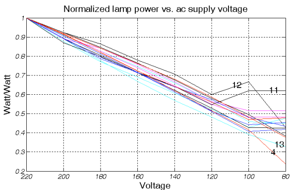
Fig. 4: Normalized lamp power vs. ac supply voltage.
