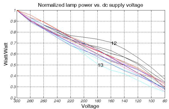
Fig. 7: Normalized lamp power vs. dc supply voltage.
