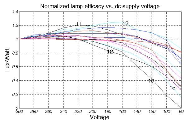
Fig. 8: Normalized lamp efficacy vs. dc supply voltage.
