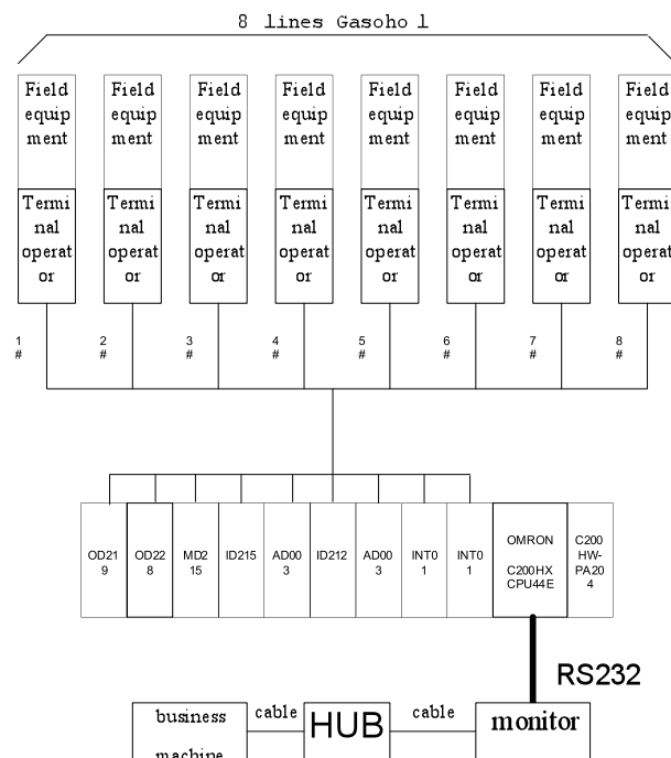
Fig.1 System structure
