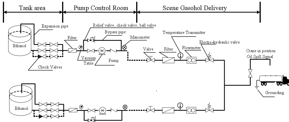
Fig.2 Single Hok-bit equipments diagram
