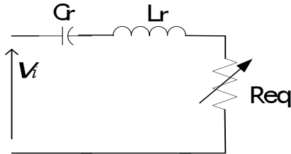
Fig. 3 Resonant tank
