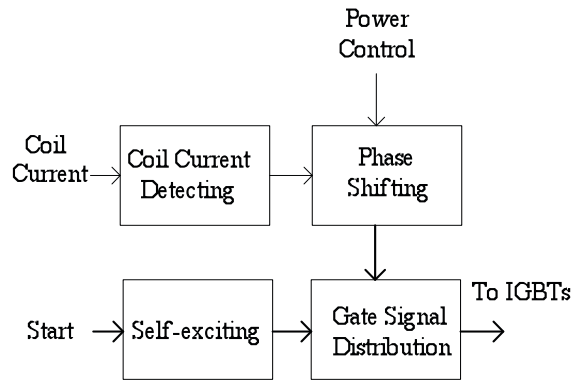
Fig. 5 Scheme of the control system
