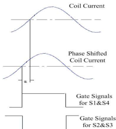
Fig. 4 Illustration of phase angle control
