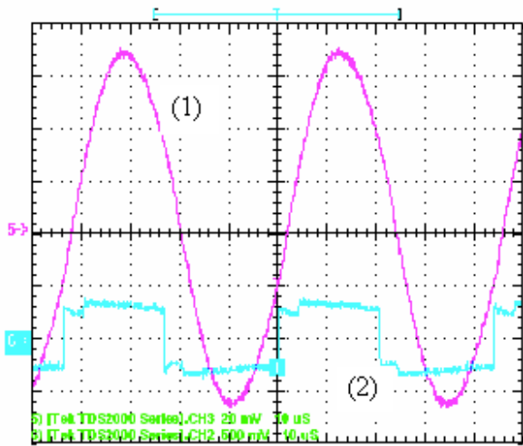
Fig. 7 Waveforms for high power (1): Coil current (2): Gate signal 20V/div 15A/DIV 10us/DIV
