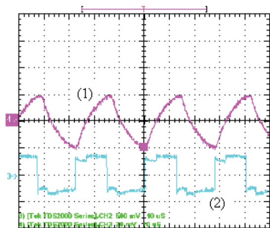
Fig. 6 Waveforms for low power (1): Coil current (2): Gate signal 10A/DIV 20V/ DIV 10us/DIV
