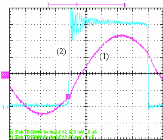
Fig. 8 Waveforms for showing ZVS (1): Coil current (2): Voltage V_A (point A) 25A/ DIV 100V/ DIV 5us/ DIV
