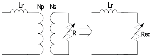
Fig. 2 Model of the coil-wok
