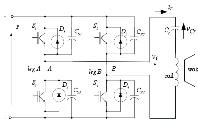
Fig. 1 Converter diagram
