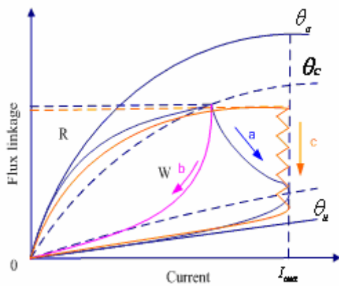
Fig. 6: Typical flux linkage waveforms.
