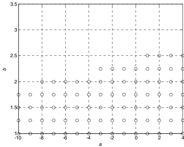
Fig. 3. Stability regions based on Theorem 3 with modification in Remark 2 and Theorem 5.
