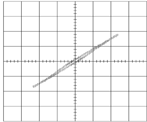
Fig. 5. Measured B - H loop of the new material poly7 ( y : 0.06 T/div, x : 13.3 kA \cdot m ^{-1} /div).
