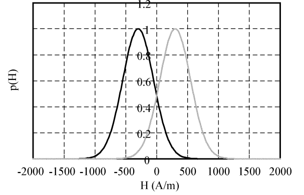
Fig. 1. Probability distribution function of the domain.
