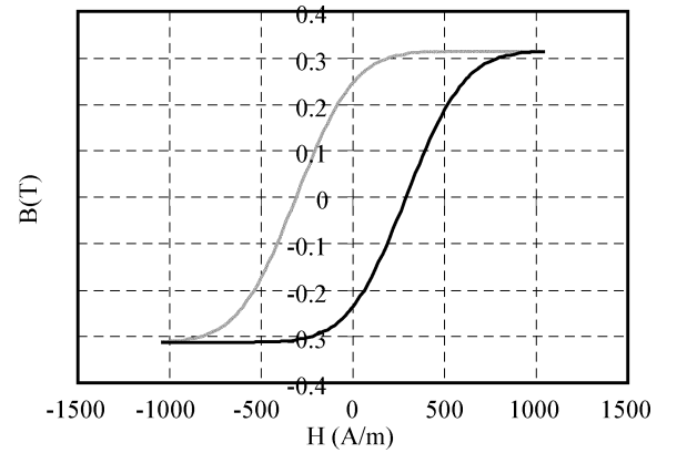
Fig. 2. B - H loop formed by the probability distribution function.
