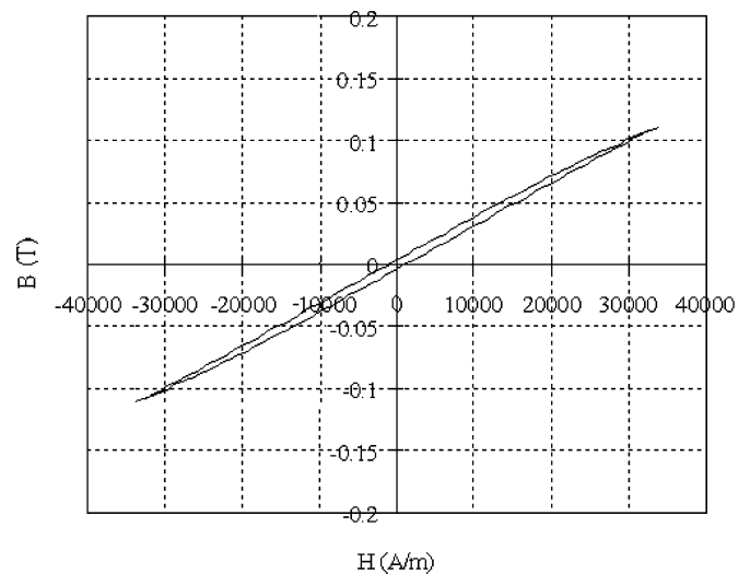
Fig. 6. Simulation of the B - H loop of material poly10.
