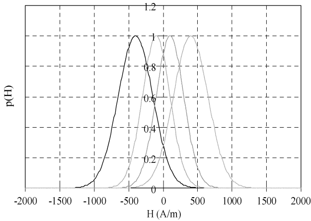
Fig. 3. Probability distribution function of domain using four orientations.
