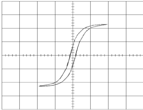
Fig. 7. Measurement of the B - H of the material 3C85 ( y : 0.1 T/div, x : 100 A \cdot m ^{-1} /div).
