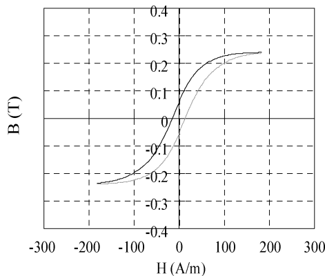
Fig. 8. Simulation of the B - H loop of 3C85.
