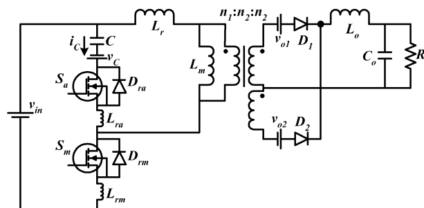
Fig. 1. Asymmetrical half-bridge forward converter.
