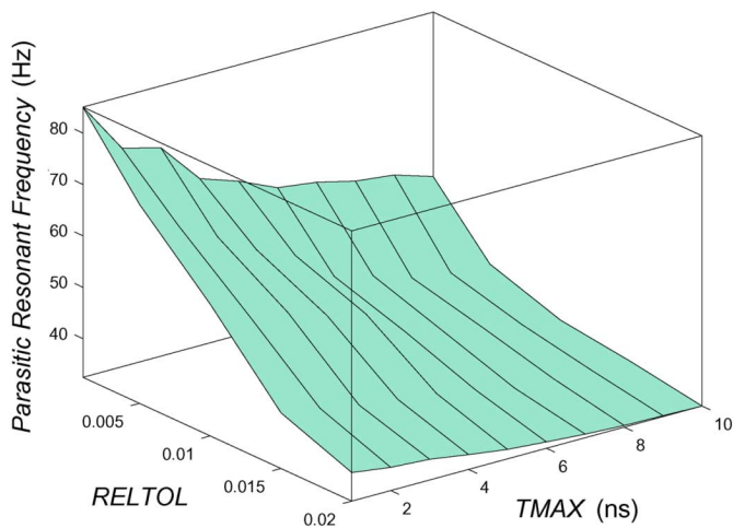
Fig. 13. Correct-flawed simulation boundary surface. "Correct" simulated results correspond to the area below the surface.
