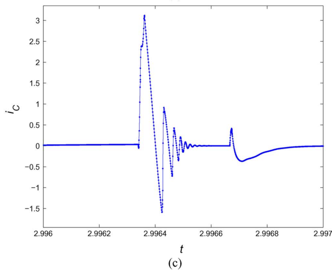
Fig. 4. (a) “Correct” simulation of i_C with RELTOL = 0.001, TMAX = 1 ns and METHOD = Gear. (b)–(c) Close-up views.
