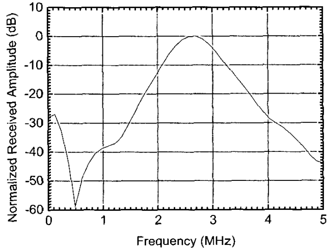
Fig. 11. Normalized received amplitude spectrum of the PMN-PT transducer.
