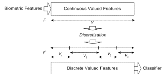
Figure 1: Discretization of biometric features to exploit class-specific dependencies.
