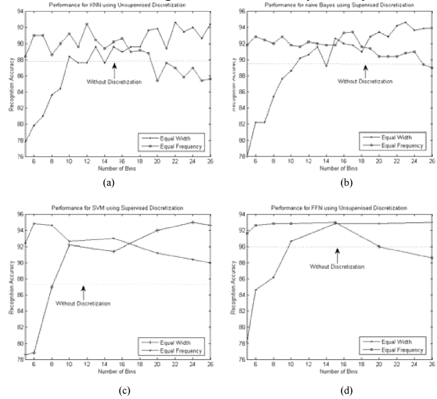
Figure 4: Performance improvement using discretization for (a) KNN, (b) naive Bayes, (c) SVM, and (d) FFN classifier.
