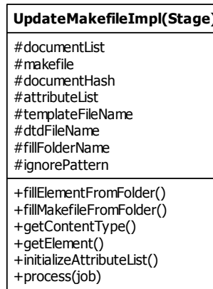
Figura 3.8 Diagrama de clases del stage build-makefile .
