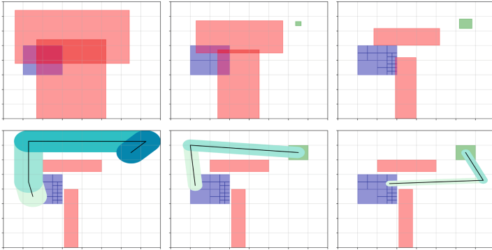
Fig. 3. Top row: each step attempting to find a reference trajectory in the space where obstacles (goal set) are bloated (shrunk) by the error bounds \{\ell_i\}_i . From left to right: \Theta is without partition, \{\ell_i\}_i are too large so a reference trajectory cannot be found. \Theta is partitioned, but \{\ell_i\}_i s for the left-top cover are still too large. With further partitions, a reference trajectory could be found. Bottom row: It is shown that the bloated tubes for each cover (which contain all other trajectories from that cover) can fit between the original obstacles.
