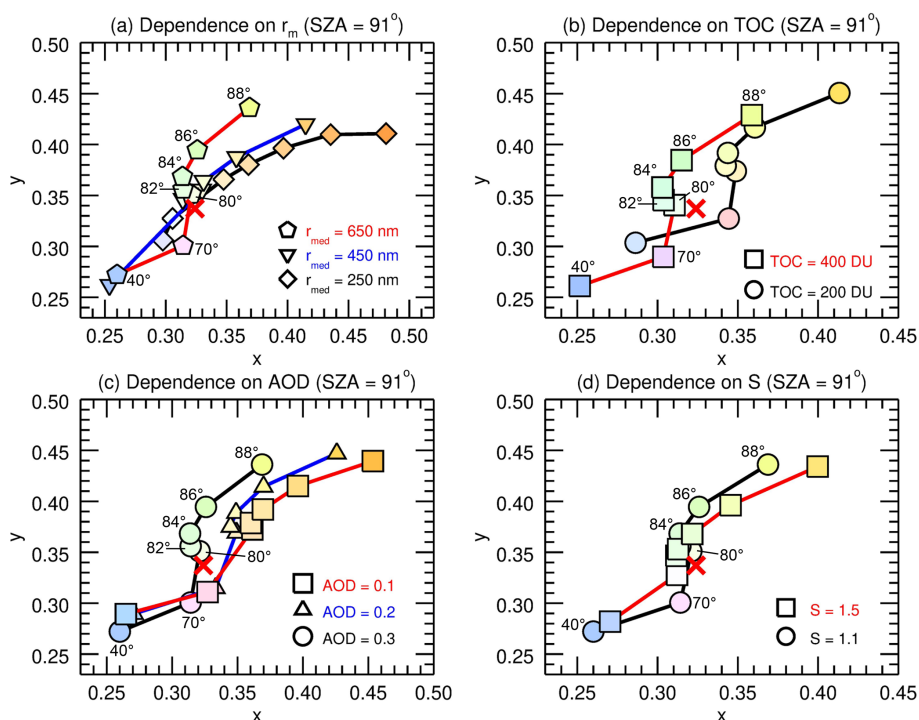
Figure 3. CIE chromaticity diagrams similar to the right panel of Fig. 2 but for variable input parameters, i.e. median radius r_{\text{med}} (a), total ozone column TOC (b), AOD (c), and width S of the PSD (d). Results are for \text{SZA} = 91^\circ , \text{SAA} = 0^\circ , and different VZAs, shown by the numbers next to the symbols in each panel (VZA values are 40, 70, 80, 82, 84, 86, and 88^\circ ). For clarity reasons, VZAs are only shown for one line in each panel.
