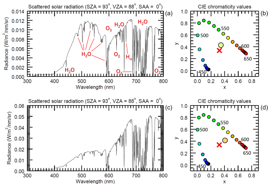
Figure 2. Spectra (a–c; note different ordinate ranges) and CIE chromaticity diagrams (b–d) for the following viewing geometry: \text{SZA} = 93^\circ , \text{VZA} = 88^\circ , and \text{SAA} = 0^\circ . The simulations shown in the top row are based on the following assumptions: \text{AOD} = 0.3 , r_{\text{med}} = 650 \text{ nm} , S = 1.1 , and \text{TOC} = 400 \text{ DU} . For the bottom row, the \text{AOD} has been set to zero and the other parameters remain the same. The “x” in the right-column panels corresponds to the chromaticity values of the unattenuated solar spectrum. The arc of the colour circles corresponds to pure spectral colours at different wavelengths (values given in nanometres with 10 nm steps) and the single-coloured circle shows the chromaticity values of the spectrum on the left.
