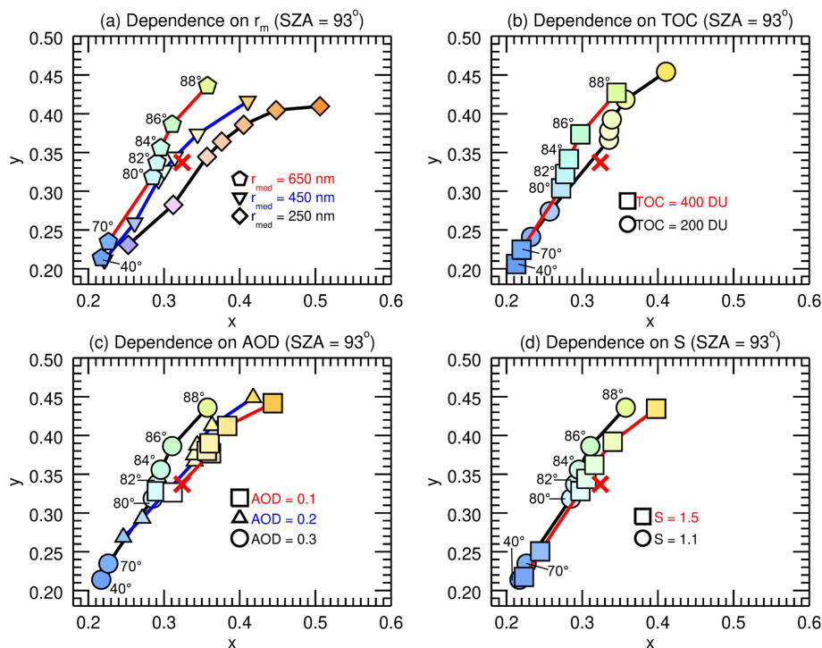
Figure 4. Similar to Fig. 2 but for SZA = 93°.
