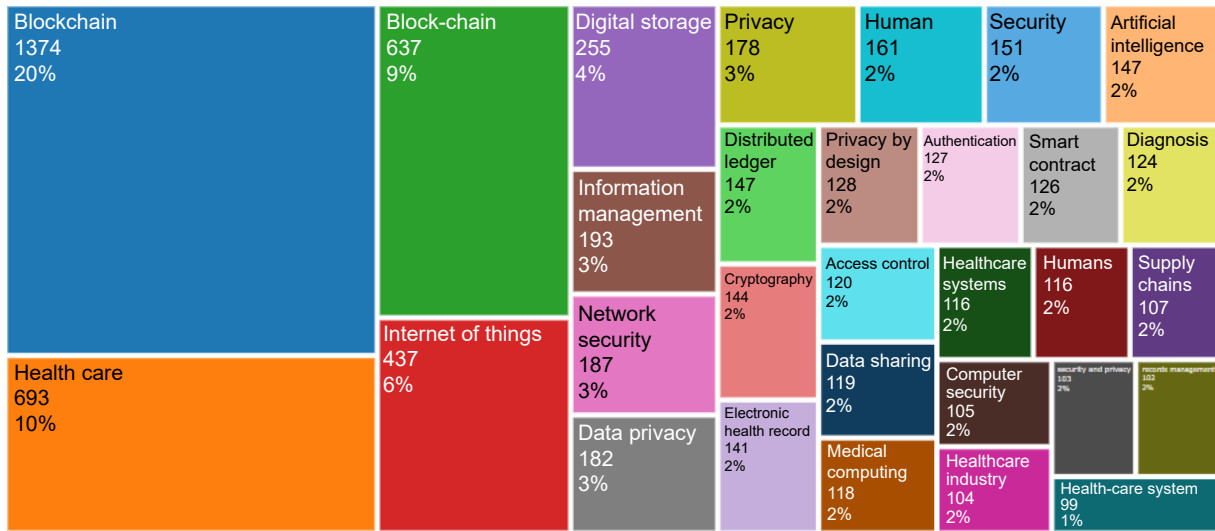
Fig. 4 Tree plot for widely used author keywords.
