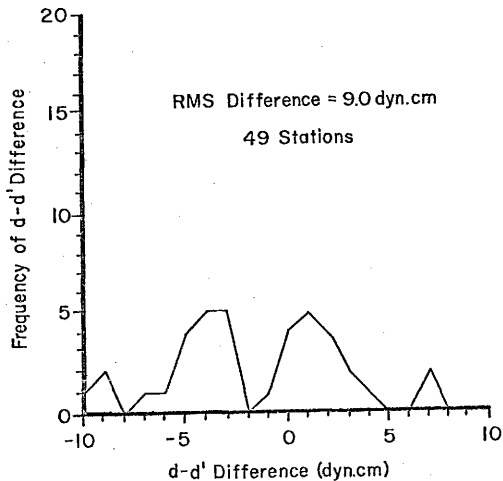
FIG. 22. Histogram of TS d-d' difference for ( 45^{\circ} - 50^{\circ} N, 165^{\circ} - 170^{\circ} W). Eleven stations have a d-d' difference that is beyond \pm 10 dyn cm.
