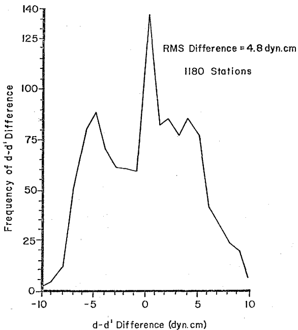
FIG. 15. Histogram of SZ d-d' difference for (30°-35°N, 160°-165°E).
