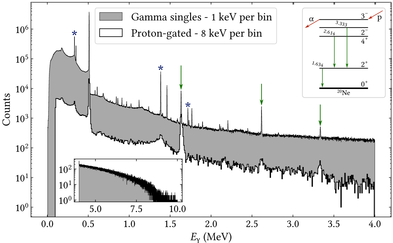
Fig. 4 Combined gamma spectra of gamma energies E_\gamma recorded in the four 4-fold segmented HPGe detectors, the high-energy part is shown in the lower inset. Both the singles and the proton-gated spectra are addback-corrected. The singles spectrum was recorded with a digital data acquisition system (DAQ) of high resolution, while the proton-gated spectrum was recorded with an analogue DAQ of lower resolution; hence the increased bin width and smaller resolution of the proton-gated spectrum. The upper inset shows the observed gamma transitions in ^{20}\text{Ne} that are marked with arrows. Note that the 2.614 MeV line coincides in energy with a background line from ^{208}\text{Tl} . The gamma lines from bound state transitions in ^{21}\text{Na} are marked by asterisks (*). See the text for further discussion.
