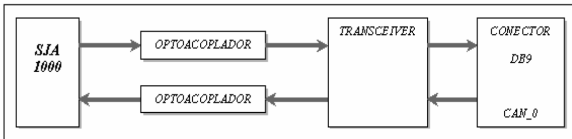
Fig. 5: Interfaz al bus CAN.
