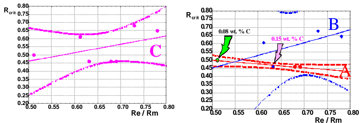
Fig. 5 Influence of design index R_e/R_m on load ratio critical value R_{crit} of selected Slovakian weldable steels and similar foreign steels with 95 % confidence interval for the specific statistics :
