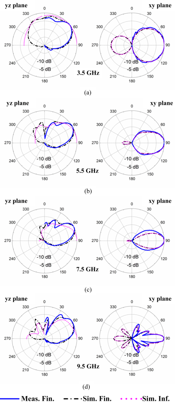
Fig. 19. Simulated and measured normalized radiation patterns in yz plane and xy plane at: (a) 3.5 GHz, (b) 5.5 GHz, (c) 7.5 GHz, and (d) 9.5 GHz.
