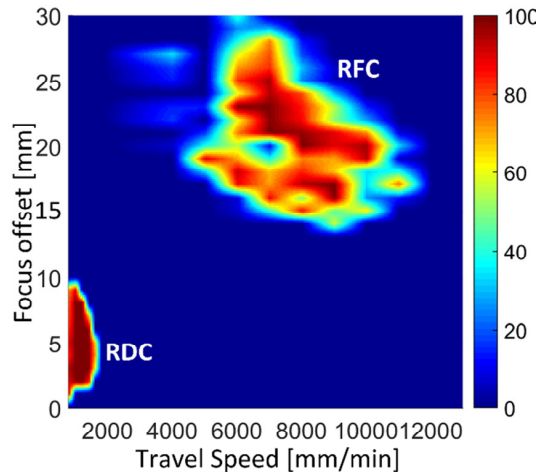
Fig. 16. The combined stability plot of RFC and remote DOE cutting (RDC). From this plot it can be seen that the stability of remote DOE cutting has a more coherent area of stability. Furthermore, the average stability in the region is close to 100% for all parameter values.
