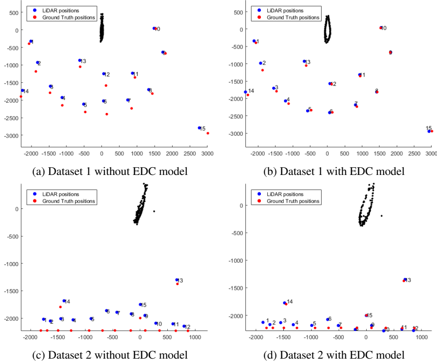
Figure 8: Localization test using the first (8a and 8b) and second(8c and 8d) position datasets. The ground truth data is shown with red dots and the LiDAR calculated positions with blue dots. The mapped blade points are also plotted, for easier orientation
