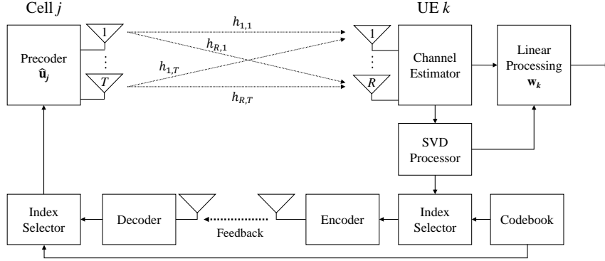
Fig. 1. Transmitter-Receiver Architecture.
