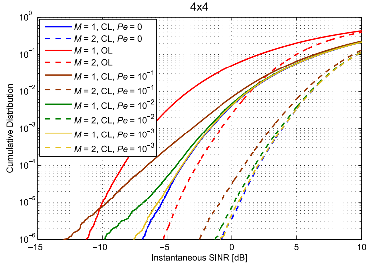
Fig. 4. SINR outage performance with a 4x4 antenna scheme, different transmission modes and precoding error probabilities ( P_e ). It is assumed that the applied PMI is known at the UE.
