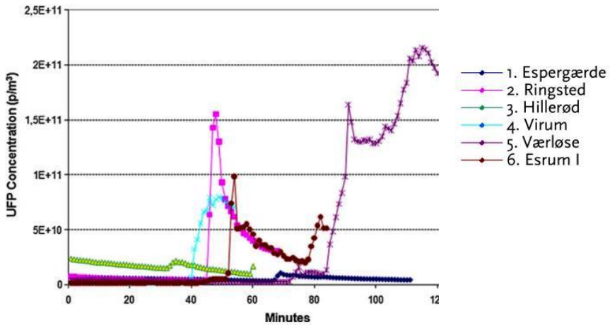
Figure 3-24 Real-time indoor concentration in number of ultra-fine particles (UFPs) per unit of air volume ( \#/m^3 ) in old and modern dwellings during the operation of thermal mass and cast-iron stoves (Paper II).
