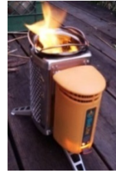
Biolite - gasifier 52 cookstove (b)
