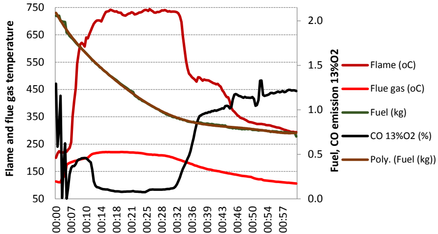
Figure 3-19 Operating conditions during the use of the wood stove equipped with the chimney retrofit by using a pre-heating system and multiple-secondary air inlets.
