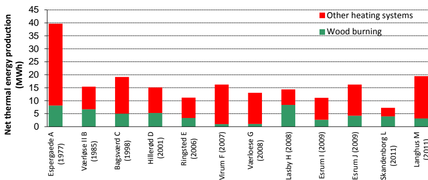
Figure 3-21 Net thermal energy production in Nordic single-family houses using masonry (Espergæde and Ringsted) and certified and cast-iron stoves.
