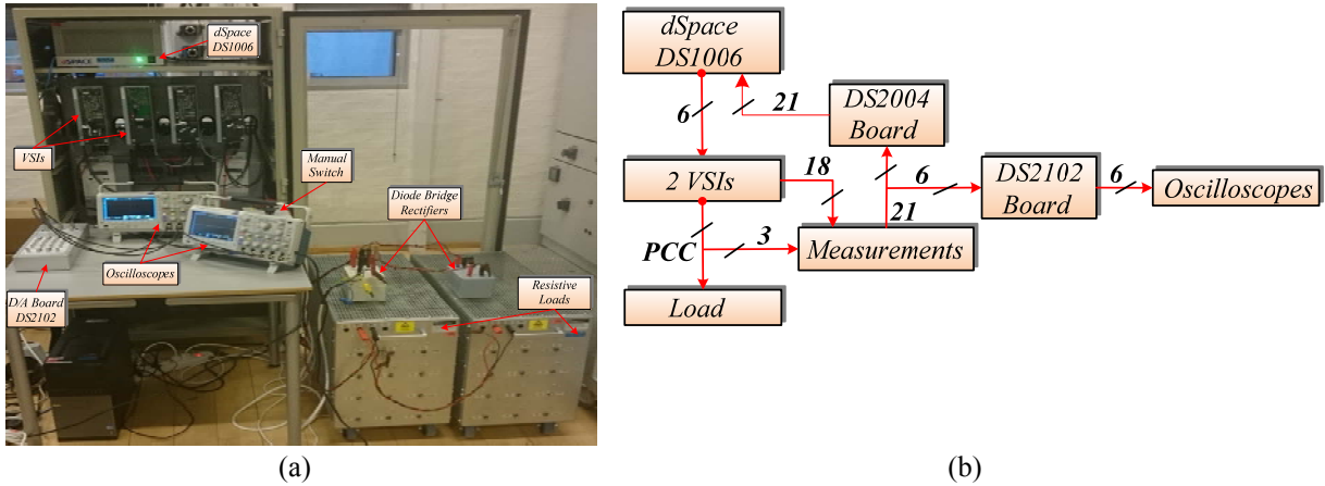
Fig. 4. (a) Photo and (b) Schematic diagram of the experimental setup
