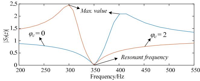
Fig. 10. Modulus of S_7(z) with different compensation angle.
