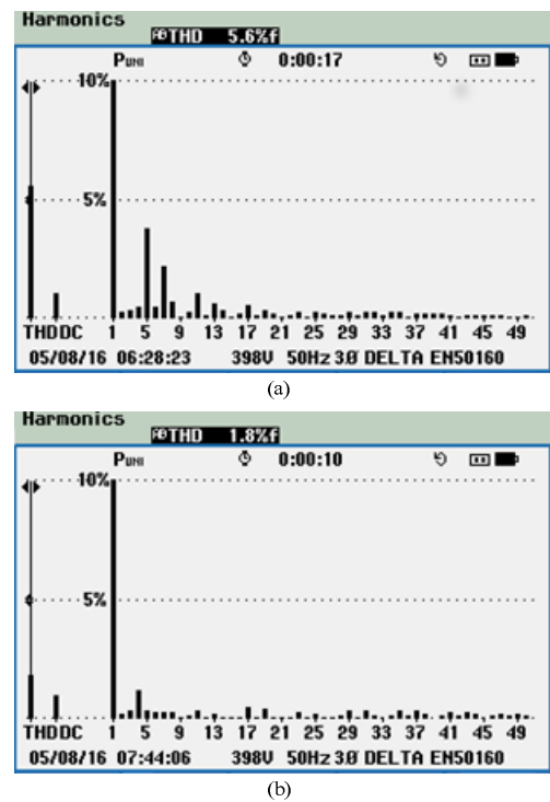
Fig. 13. PCC voltage spectrum and THD. (a) before compensation. (b) after compensation.
