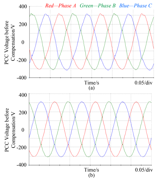
Fig. 12. PCC voltage. (a) before compensation. (b) after compensation.
