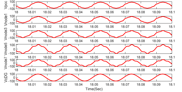
Fig.11 Voltage distortion along the feeder without harmonic damping
