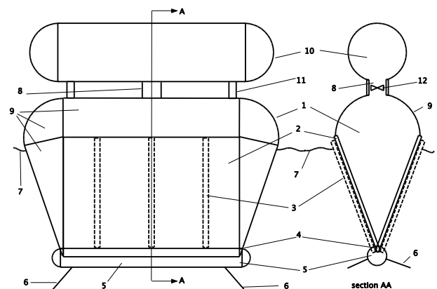
Fig. 1 The free floating clam device, reproduced from [3, 4]
