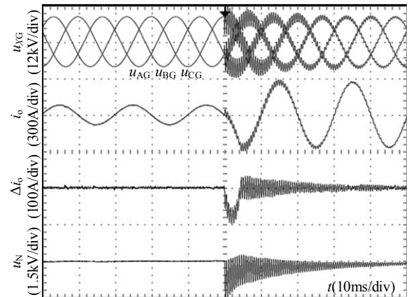
Fig. 17. Dynamic waveforms subjected to load step-up from 30% nominal load to 100% with proposed method.
