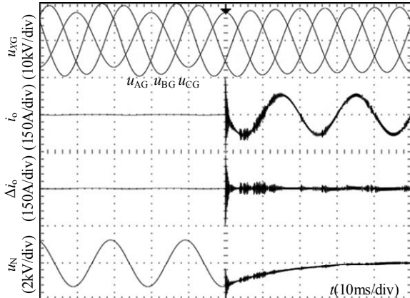
Fig. 14. Dynamic waveforms subjected to load step-up from 0 to 30% nominal load with PI controller.
