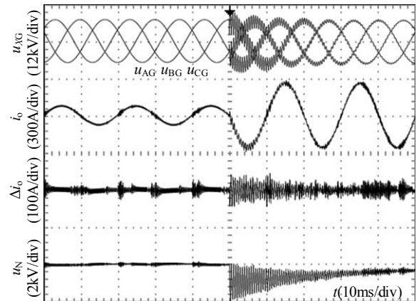
Fig. 16. Dynamic waveforms subjected to load step-up from 30% nominal load to 100% with PI controller.
