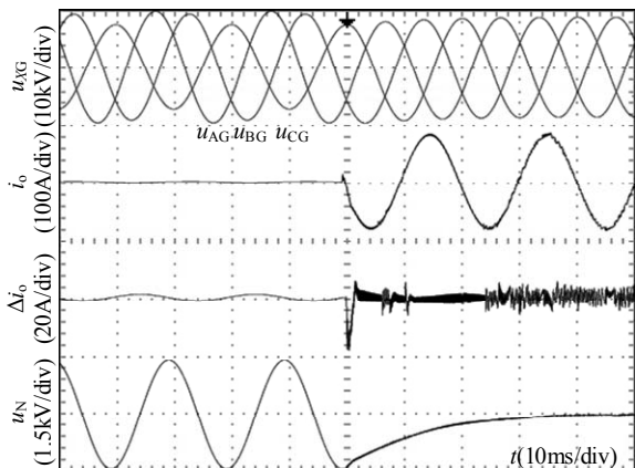
Fig. 15. Dynamic waveforms subjected to load step-up from 0 to 30% nominal load with proposed method.
