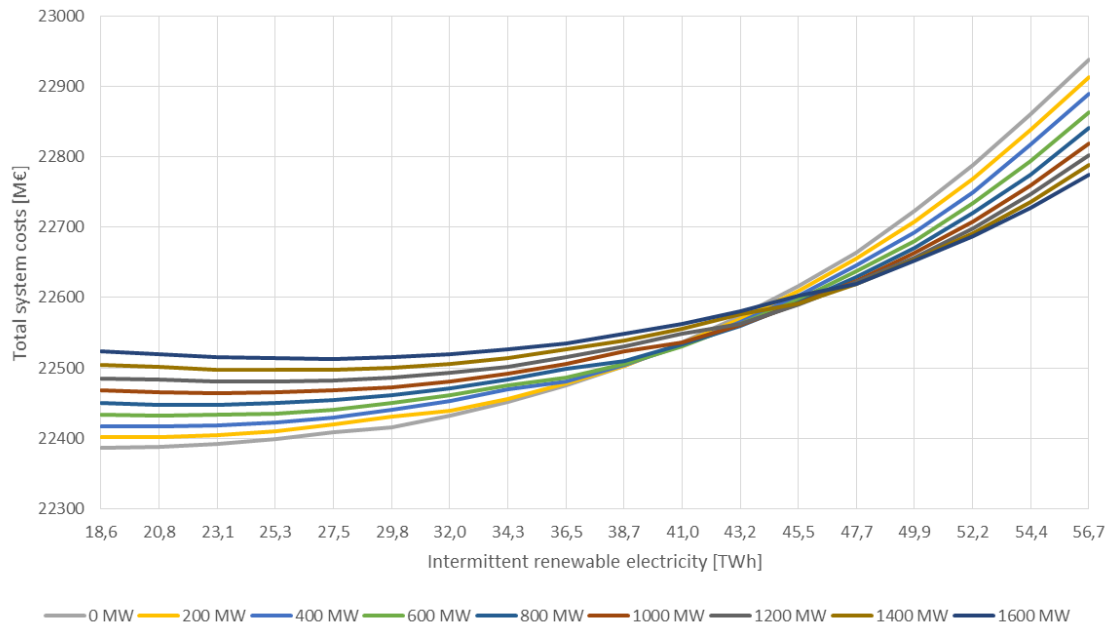
Figure 18. Total system costs for electrofuel production with different alkaline electrolyser capacities and increasing wind capacity
