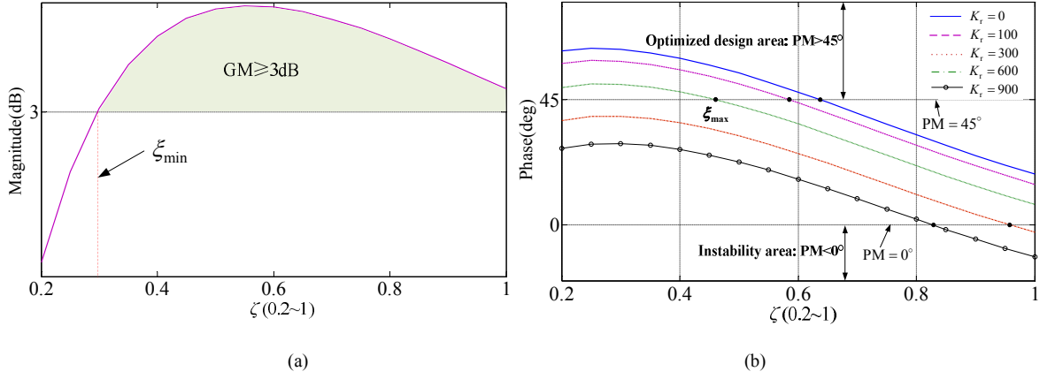
Fig.7. The PM and GM of the open loop with \zeta . changing. (a) The relationship between GM and \zeta . (b) The relationship between PM and \zeta .
