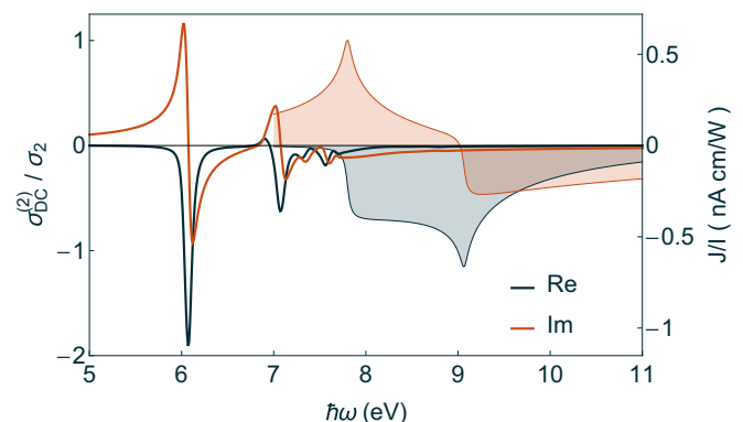
FIG. 11. Photoconductivity of a hBN monolayer with excitonic corrections. Model parameters are identical to those in Fig. 3. The shadowed curves reproduce the independent-particle results shown in Fig. 3, vertically scaled up by a factor of 10.
