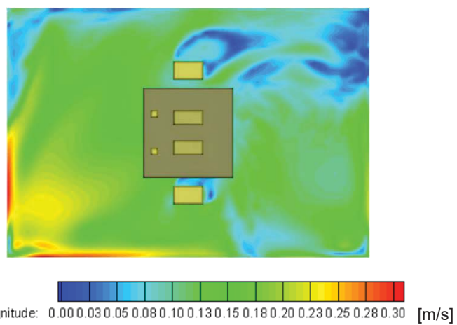
Fig. 18. Velocity distribution at a height of 0.1 m with the square opening
