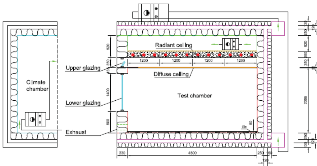
Fig.2. Vertical section view of environmental chamber
