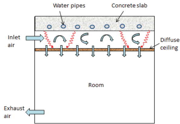
Fig.1 Schematic diagram of the integrated system
