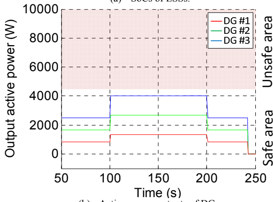
(b) Active power outputs of DGs.
