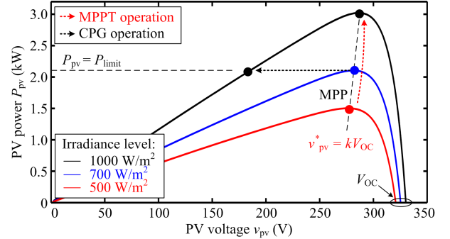
Fig. 4. Operational principle of the PV side control scheme, where the Constant Voltage MPPT and the CPG algorithms are implemented.
