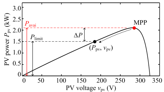
Fig. 2. Power-voltage curve of the PV panels with the reserved power control.
