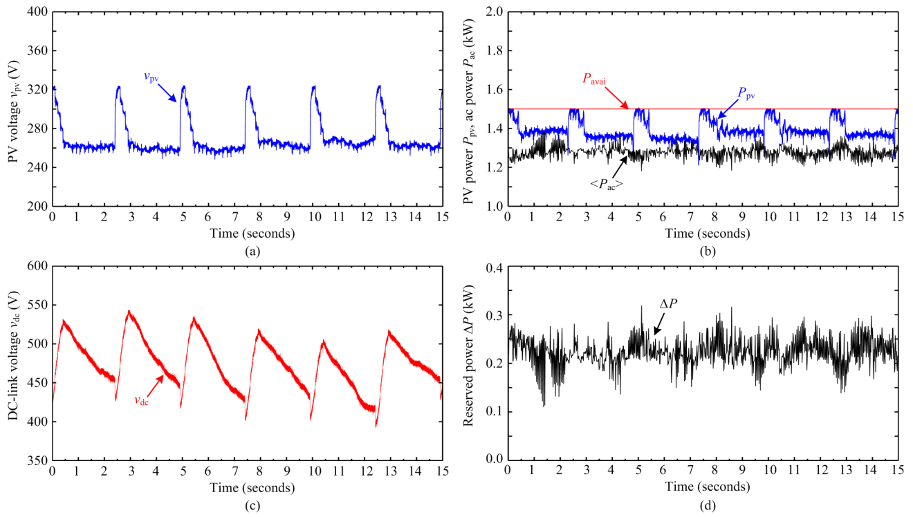
Fig. 11. Zoomed-in view of the results in Fig. 10: (a) PV voltage v_{pv} , (b) PV power P_{pv} and ac power P_{ac} , (c) dc-link voltage v_{dc} , (d) reserved power \Delta P .
