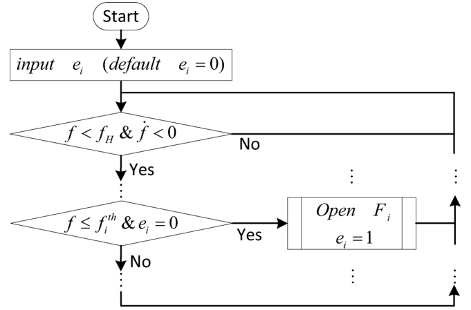
Fig. 1. Flowchart of the proposed LS scheme.
