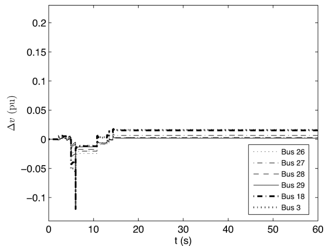
Fig. 9. Scenario 2: the voltage deviation from v_{ss} (AUFVLS).
