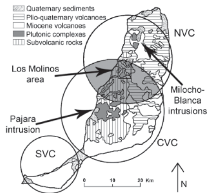
Figure 1.- Geological sketch of Fuerteventura with location of the main intrusive bodies and three major Miocene volcanoes reconstructed by Ancochea et al. (1996). NVC: Northern Volcanic Complex. CVC: Central Volcanic Complex. SVC: Southern Volcanic Complex.
