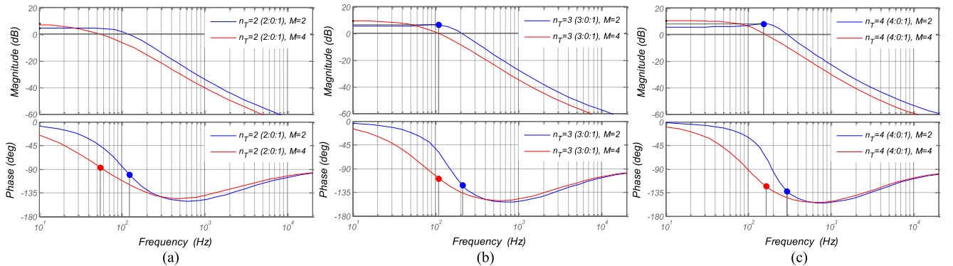
Fig. 22. Bode plot for input to capacitor voltage transfer function of PWM T-source converter with various turns ratios and voltage gains.
