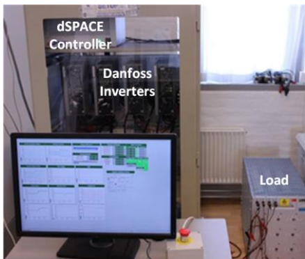
Fig. 6. Experimental setup
