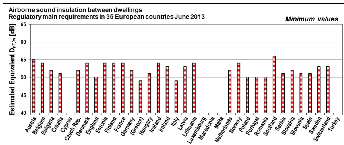
Figure 3 – Overview of airborne sound insulation requirements between dwellings. Status 2013. Graphical presentation of estimated equivalent values of D_{nT,w} . Note: The equivalent values are estimates only, as exact conversion is not possible. Figure from [10].
