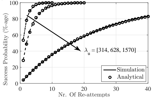
Fig. 4: Cumulative Success Probabilities after n^{\text{th}} re-attempt for \rho = 0.1 with the singleton approach and \lambda_u = [314, 628, 1570] users.
