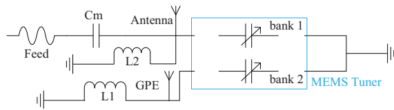
Fig. 1: Antenna and GPE tuning concept: the tank circuit combining L2 and bank 1 of the MEMS tunes the antenna; L1 and bank 2 of the MEMS tune the GPE. The fixed capacitor C_m matches the antenna to the feed line. There is no connection between the feed line or the antenna and the GPE.
