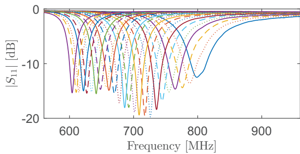
Fig. 6: Return loss of design A when the 1040 MEMS tuner varies from 0.5 pF to 6.5 pF in steps of 0.25 pF.
