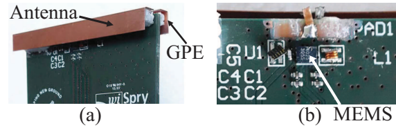
Fig. 5: Demonstrator board. (a) Demonstrator with the antenna and the GPE mounted. (b) Detailed view of the matching and tuning network for design B. The MEMS tuner (U1) has two independent banks, one for controlling the antenna and one for controlling the GPE.
