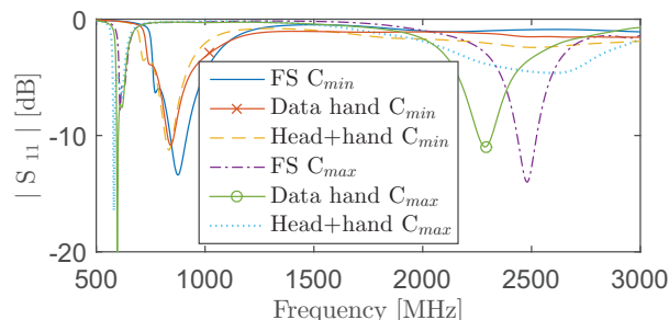
Fig. 10: Return loss in free space, in the presence of the user phantom in talk mode (Fig. 9a) and in the presence of the user hand in data mode (Fig. 9b).
