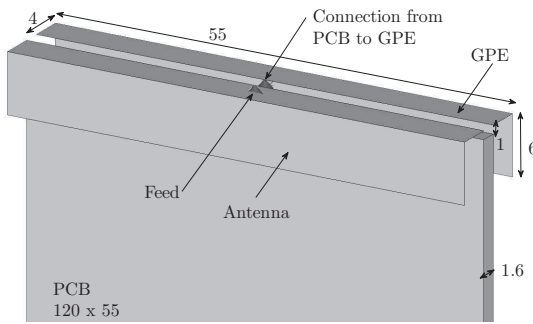
Fig. 4: Antenna and GPE geometries (dimensions in mm).
