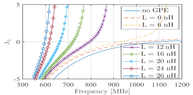
Fig. 3: Eigenvalues of the first mode ( \lambda_1 ) of the tuned ground plane.
