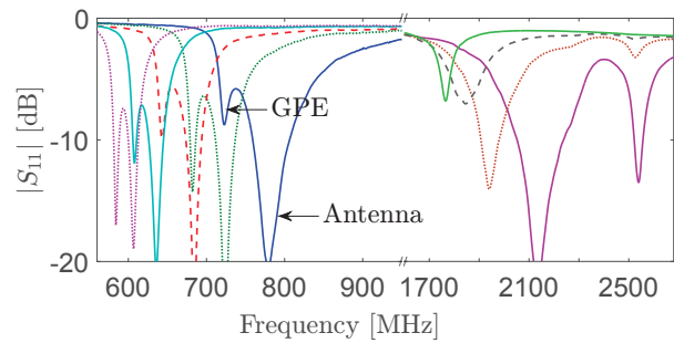
Fig. 8: Return loss of design B in the low and high bands of the LTE spectrum where the tuner varies according to IV-C.
