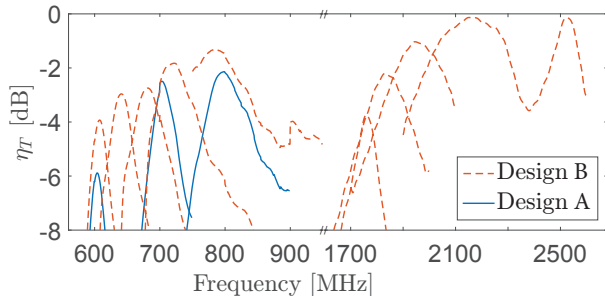
Fig. 7: Total efficiency of design A (without GPE) for minimum, medium and maximum capacitance of the 1040 MEMS tuner in the low bands, and of the design B (with GPE) when the 1040 MEMS tuner varies according to IV-C.
