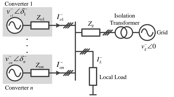
Fig. 9. Negative sequence equivalent circuit.
