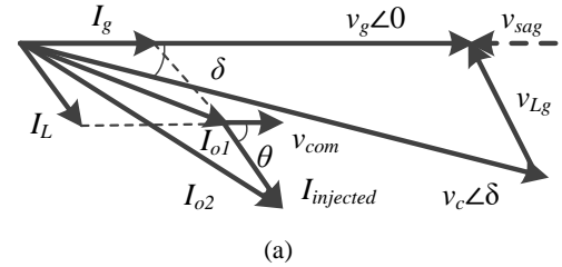
Fig. 4. Steady-state phasor diagram with only reactive current injection under complex line impedance condition.
