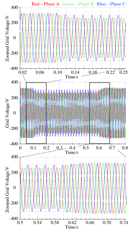
Fig. 23. Grid voltage with a two-phase 0.2 p.u. sag.
