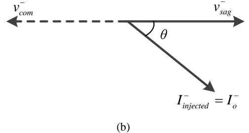
Fig. 5. Steady-state phasor diagram with both active and reactive current injection under complex line impedance condition. (a) positive sequence diagram and (b) negative sequence diagram.
