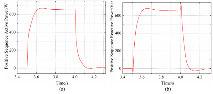
Fig. 20. Positive sequence output power of the converter. (a) active power and (b) reactive power.
